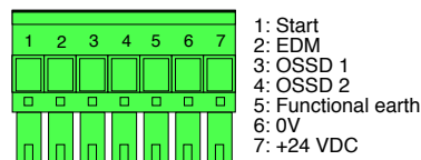
Connection of PLSG 3 corresponds to BLVTE
