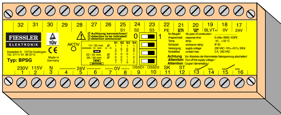
Programming and control unit BPSG
