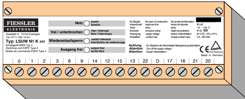
LSUW N1 K 24 VDC version
