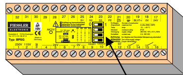
Dip switch for setting the blanking mode
