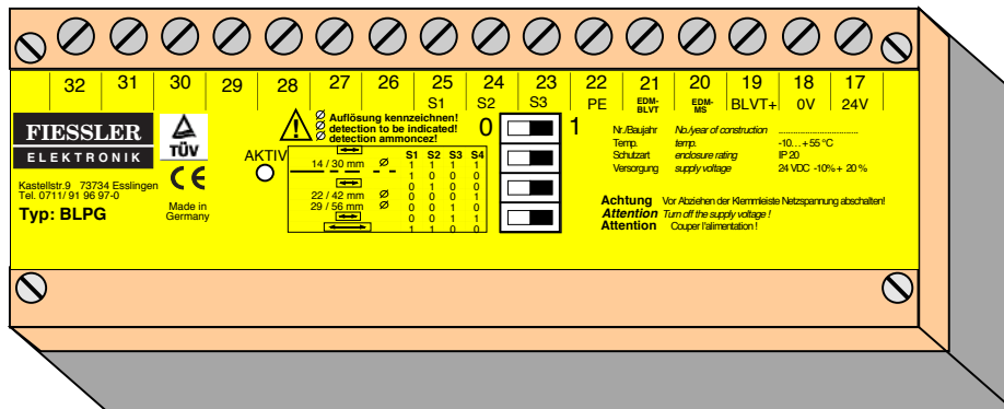
Programming unit BLPG
